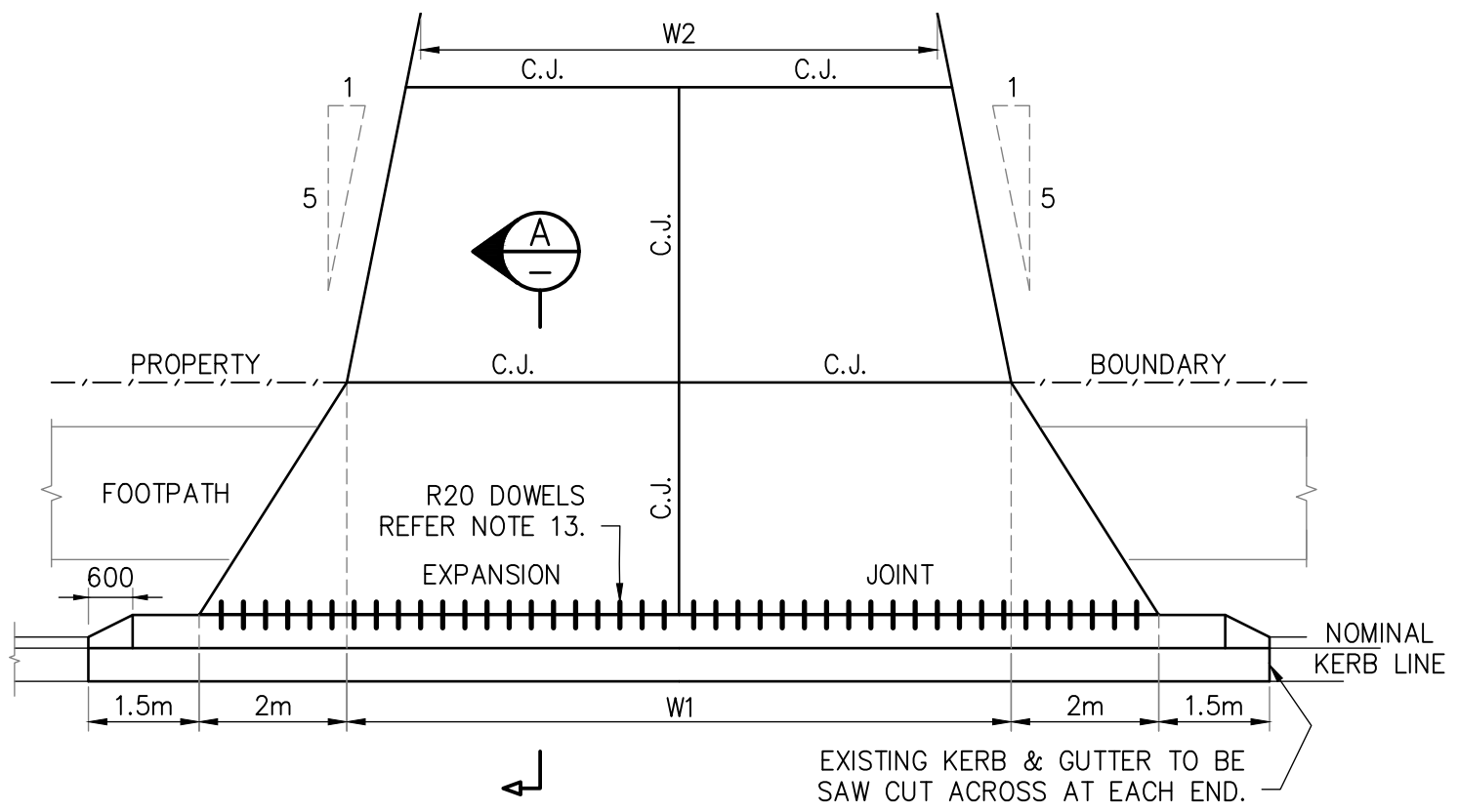
PLAN SCALE 1:100
